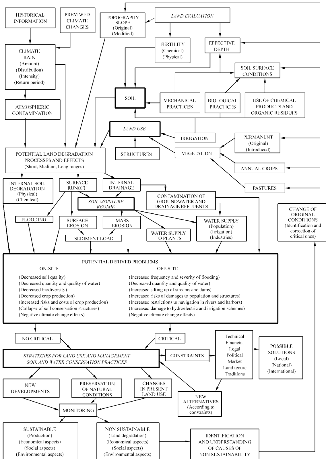
Fig.2 Interactions of land degradation processes, causes and effects, with land use, management and soil and water conservation practices
