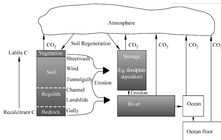
Fig.1 Mass balance approach being used to assess how much eroded C is sequestered annually in land and marine environments and lost annually to the atmosphere as CO 2 . This study is focussed on reporting on potential sources and sinks of erosion-related C in the terrestrial environment. The size of arrows indicating CO 2 fluxes are not related to their magnitude.
