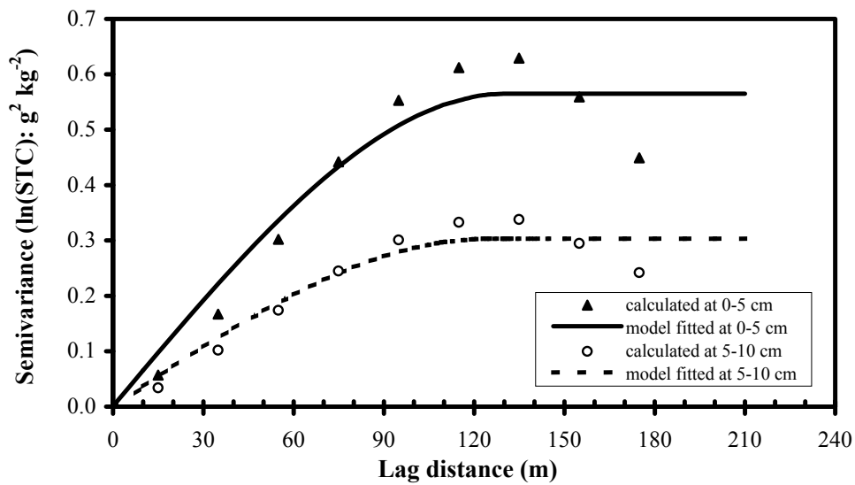
Figure 4. Semivariograms of \ln(\text{STC}) at two depths.
