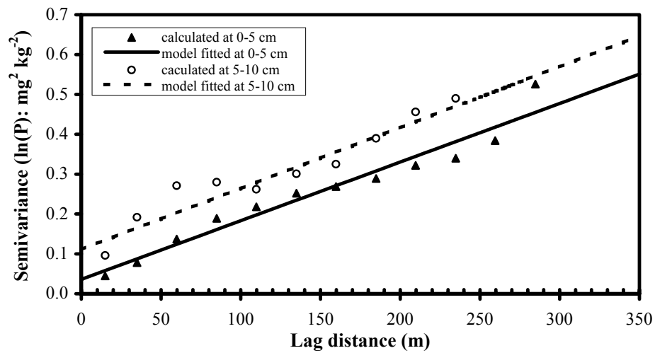
Figure 3. Semivariograms of \ln(P) at two depths.
