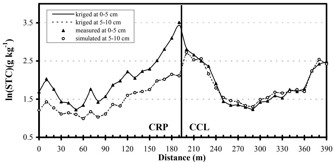
Figure 7. One dimensional \ln(STC) distribution at two depths: measured vs kriged
