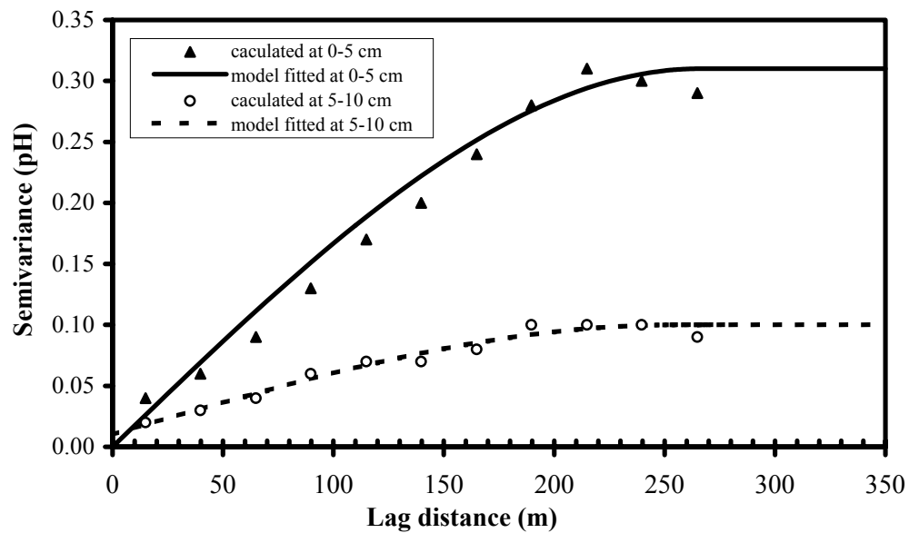
Figure 2. Semivariograms of soil pH at two depths.
